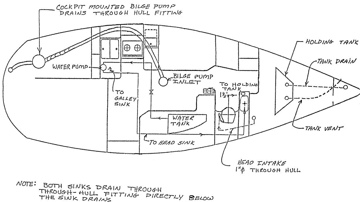
Figure 5 - General Plumbing Schematic
